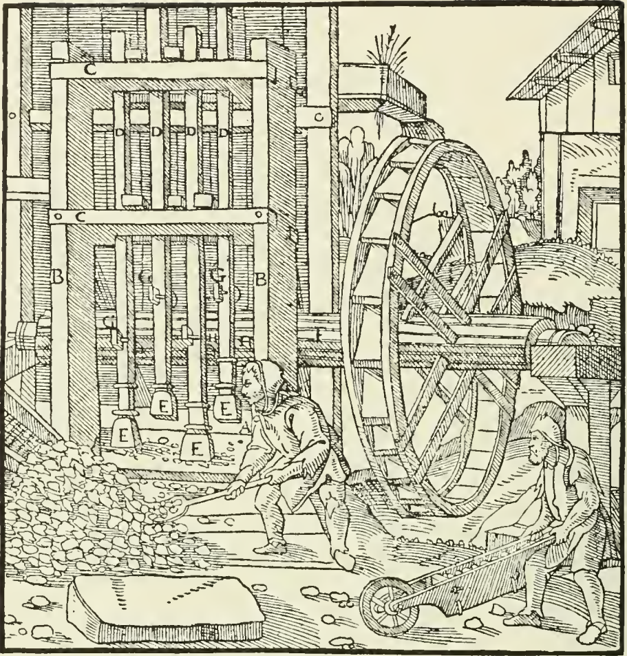
A—MORTAR. B—UPRIGHT POSTS. C—CROSS-BEAMS. D—STAMPS. E—THEIR HEADS. F—AXLE (CAM-SHAFT). G—TOOTH OF THE STAMP (TAPPET). H—TEETH OF AXLE (CAM).
